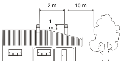
(1) The chimney cap must not show hindrances within 10 m from walls, pitches and trees. Otherwise raise it of at least 1 m over the hindrance. The chimney cap must exceed the ridge of the roof of at least 1 m.
